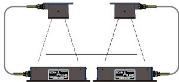
Model 10XAS-10E-B Dual-Sensor System
