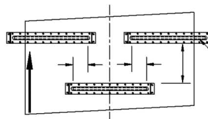
Multiple sensors for wide strip & variable hole locations
